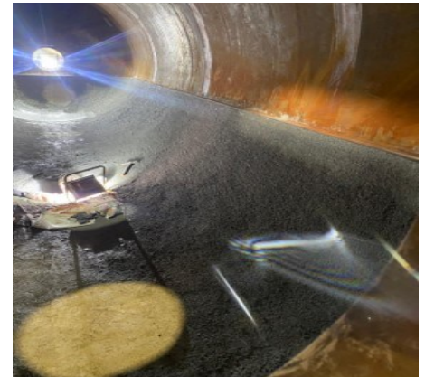
ACID GUARD PC Sulfur Train Knock Out Drum
