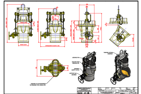
Engineering drawing of ladle
