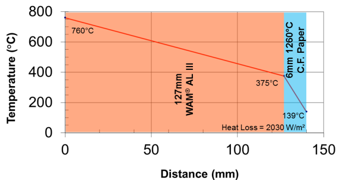
WAM® AL III Steady State Heat Flow with Heat Loss
